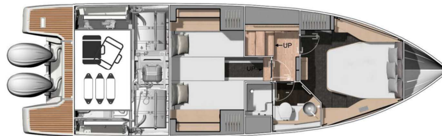
2 cabines • 1 Salle de bain • Breakfast Point / 2 cabins • 1 Head • Breakfast Point Version hors-bord / Outboard version
